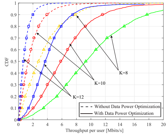
Figure 4. CDFs of the per-user throughput for the cases of uplink data transmission power optimization and without power optimization, K = 8, 10, 12, A = 15, M = 1 , and \tau^p = 10 .
