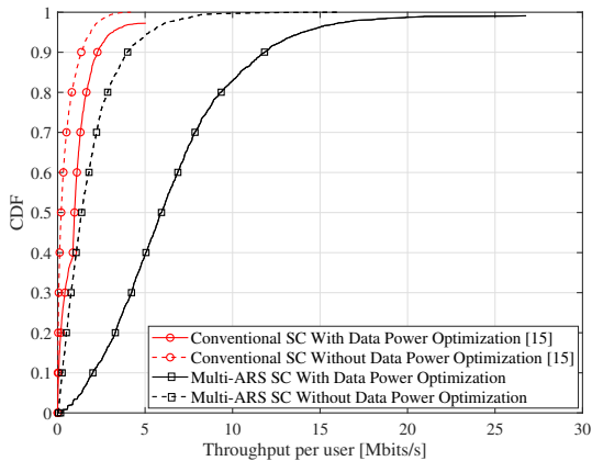
Figure 3. CDFs of the per-user throughput for the cases of conventional SC and Multi-ARS SC, K = 10, A = 15, M = 1 , and \tau^p = 10 .
