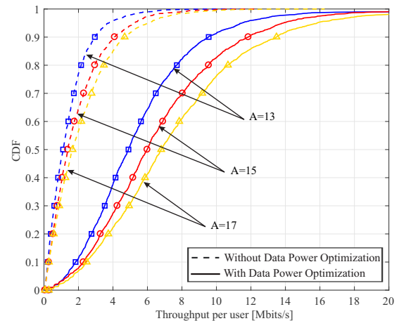
Figure 5. CDFs of the per-user throughput for the cases of uplink data transmission power optimization and without power optimization, A = 13, 15, 17, K = 10, M = 1 , and \tau^p = 10 .
