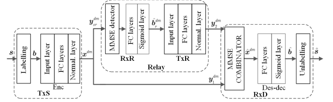
Figure 5. The AE-DF system using MMSE combinator.
